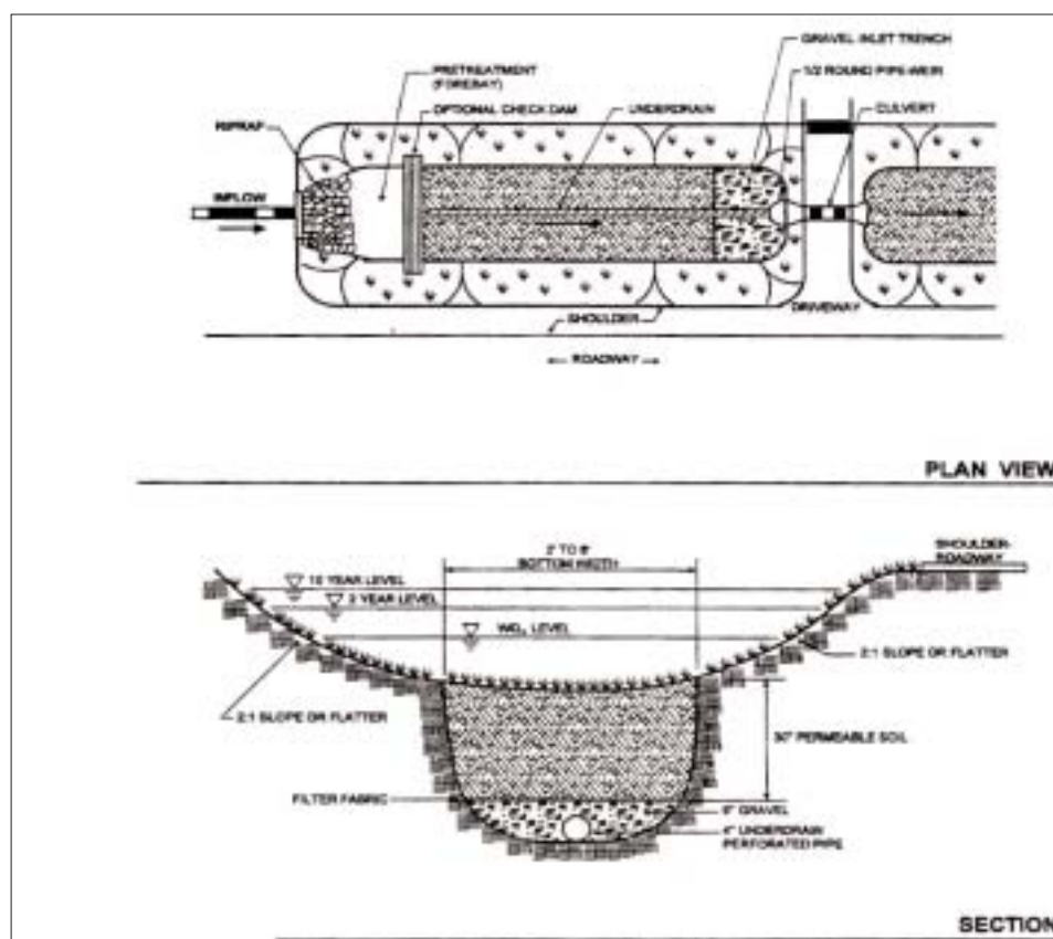
Dry swale design (Diagram: Prince George's County, MD- Low Impact Design Strategies)
