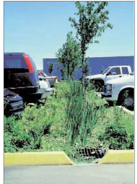
Parking median bioretention with curb cut (Photo: Portland Bureau of Environmental Service)
