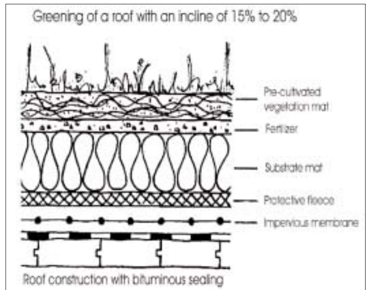
Green roof cross section (Drawing: Prince George's County LID Design Guide)
